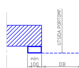
KKR 100x50x4
