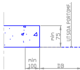
BETONG
