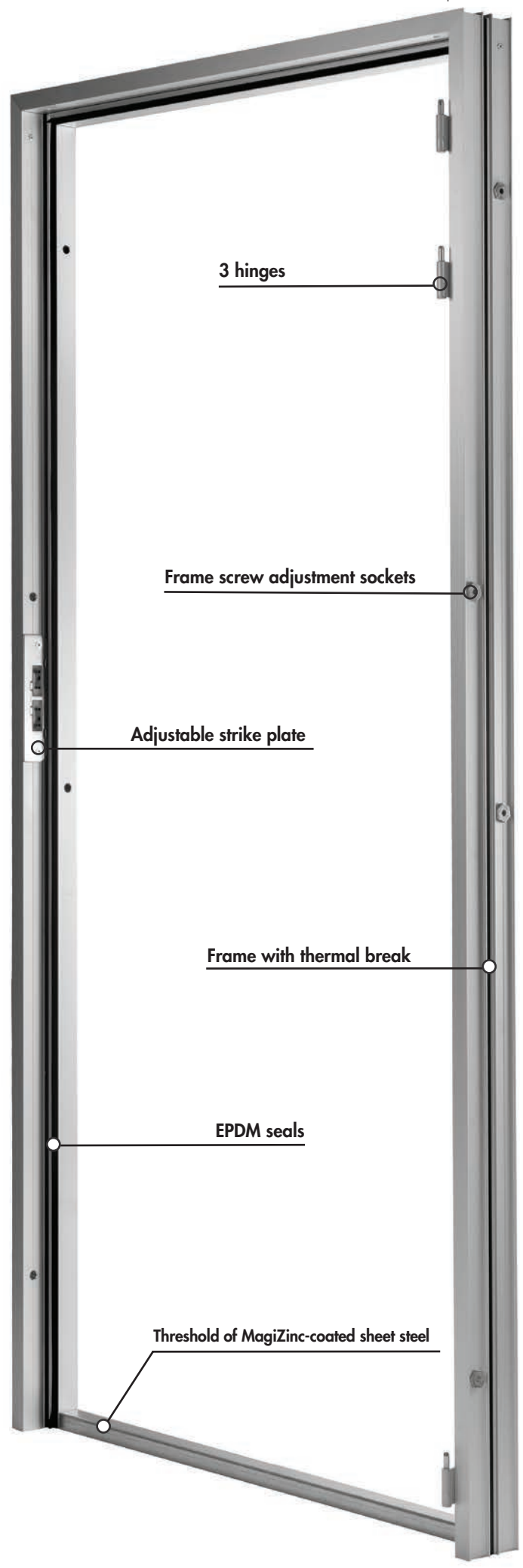
Frame with thermal break
