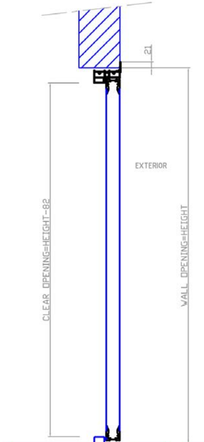
Vertical section
