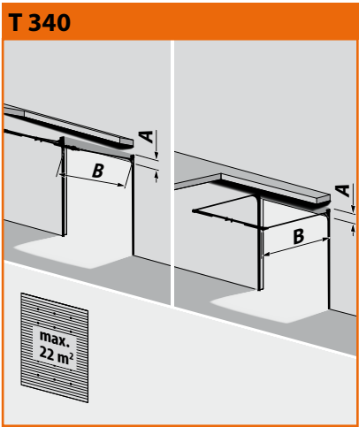
T 340 Standard rail system, rear suspension package + steel support profile A= 340 mm B= open width + 750 mm Width max. 6,500 mm
