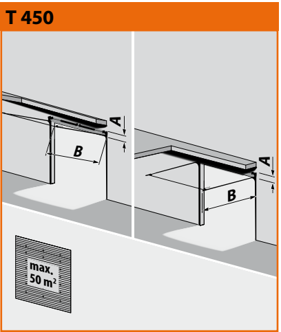
T 450 Standard rail system (comes standard) A = 430-510 mm B= open height + 650 mm
