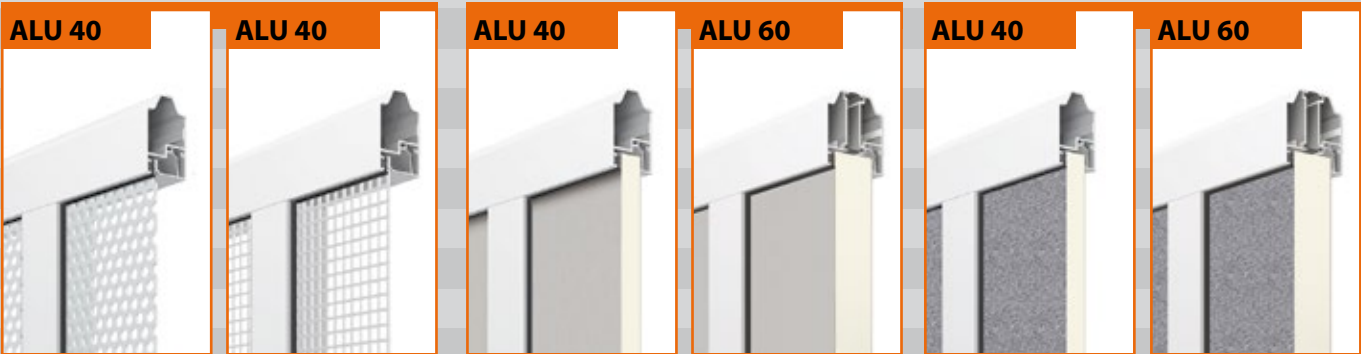
Single-walled perforated ALU plate (2 mm) round perforation (air transmittance 40%) ALU 40 (2 mm) square perforation (air transmittance 70%) Double-wall closed sandwich version (20 mm), smooth plate on the outside and plaster on the inside ALU 60 (40 mm), smooth plate on the outside and plaster on the inside Double-wall closed sandwich version (20 mm), plaster on the inside and outside ALU 60 (40 mm), plaster on the inside and outside
