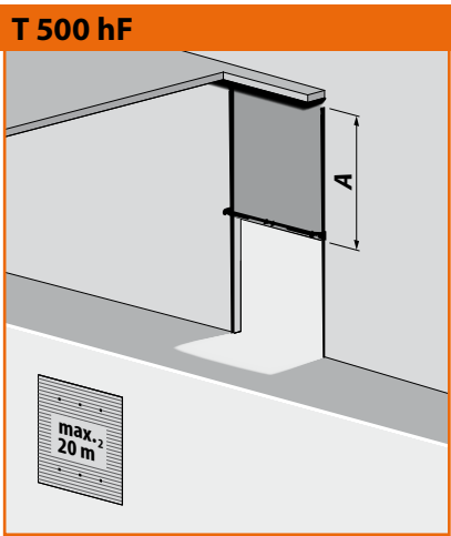
T 500 hF Vertical rail system with low spring axis + steel support profile A= open height + 400 mm Width max. 4,500 mm
