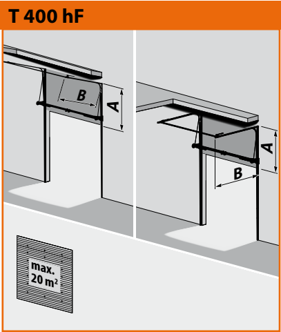
T 400 hF Elevated rail system with low spring axis + steel support profile A= hoisting + 200 mm B= open height – hoisting + 600 mm Width max. 4,500 mm Lift min. 1,450 mm
